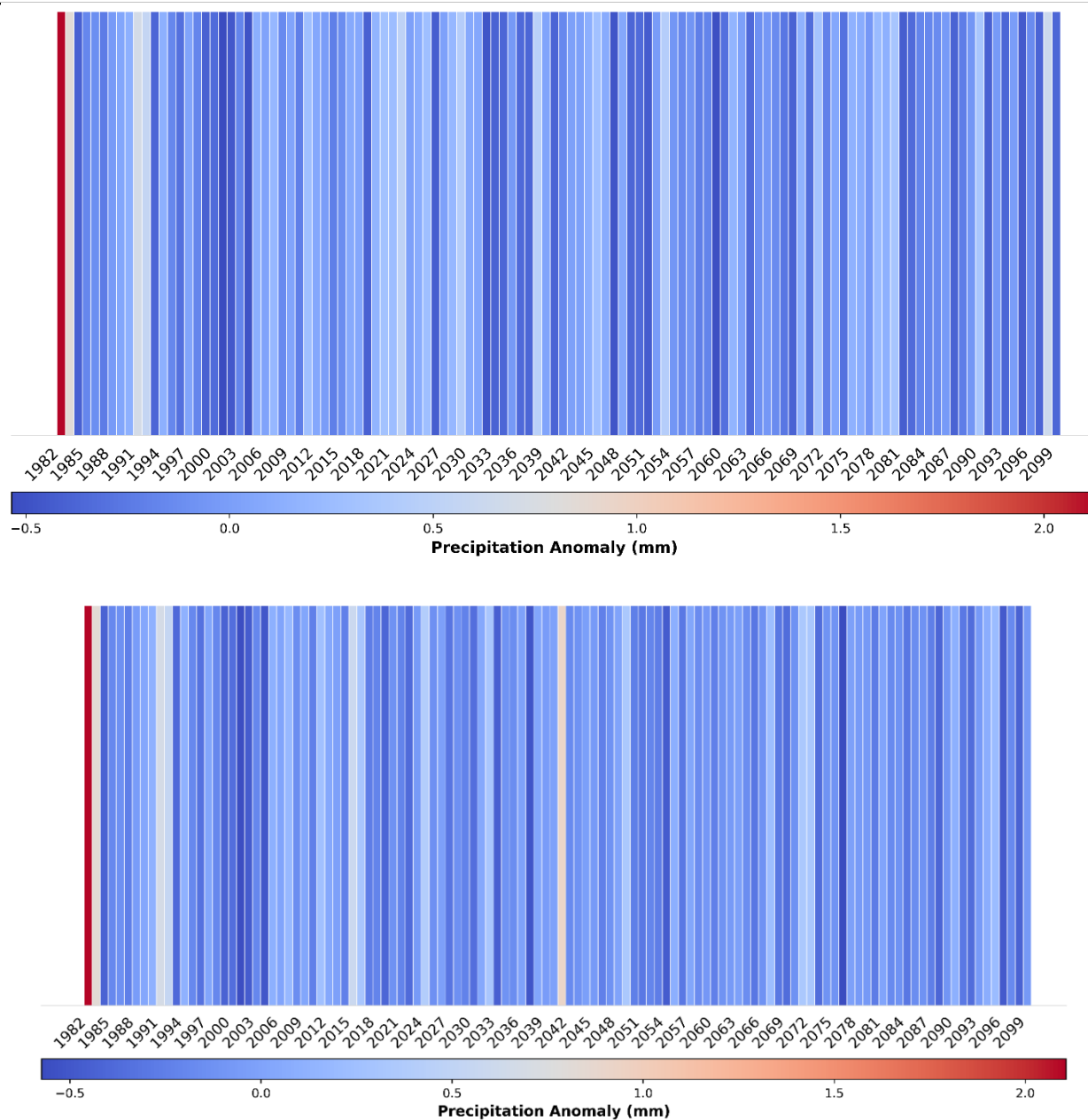
Figure 12 | Anomaly in precipitation under (a) SSP245 and (b) SSP585 scenarios.
